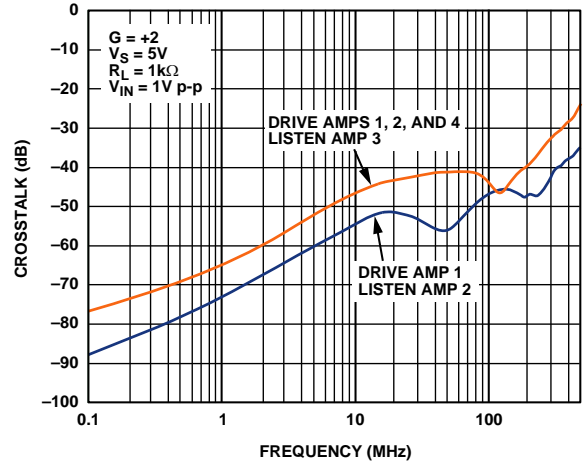
Figure 38. ADA4851-4, RTI Crosstalk vs. Frequency
